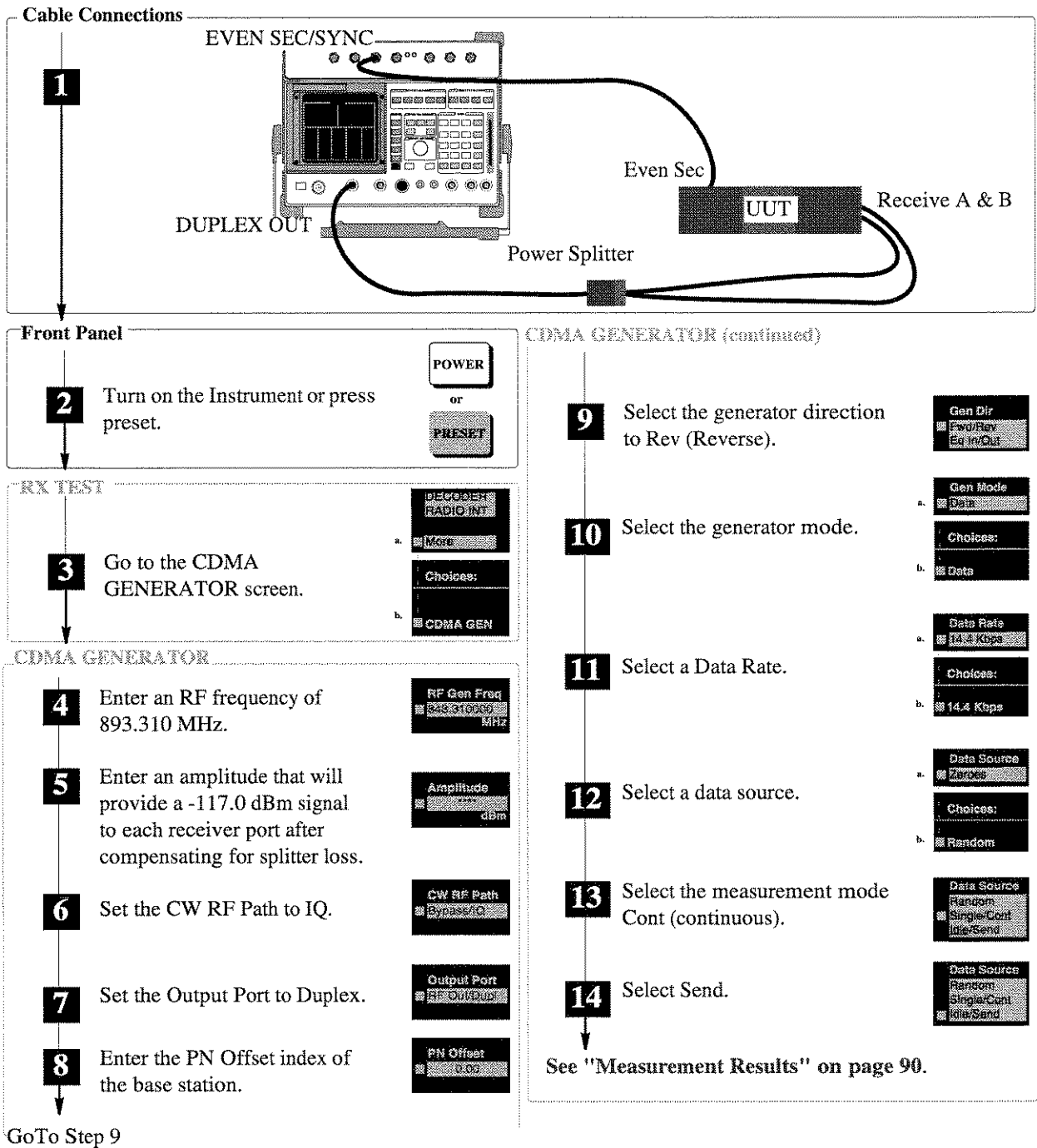
Figure 7 Receiver Sensitivity Measurement Procedure
