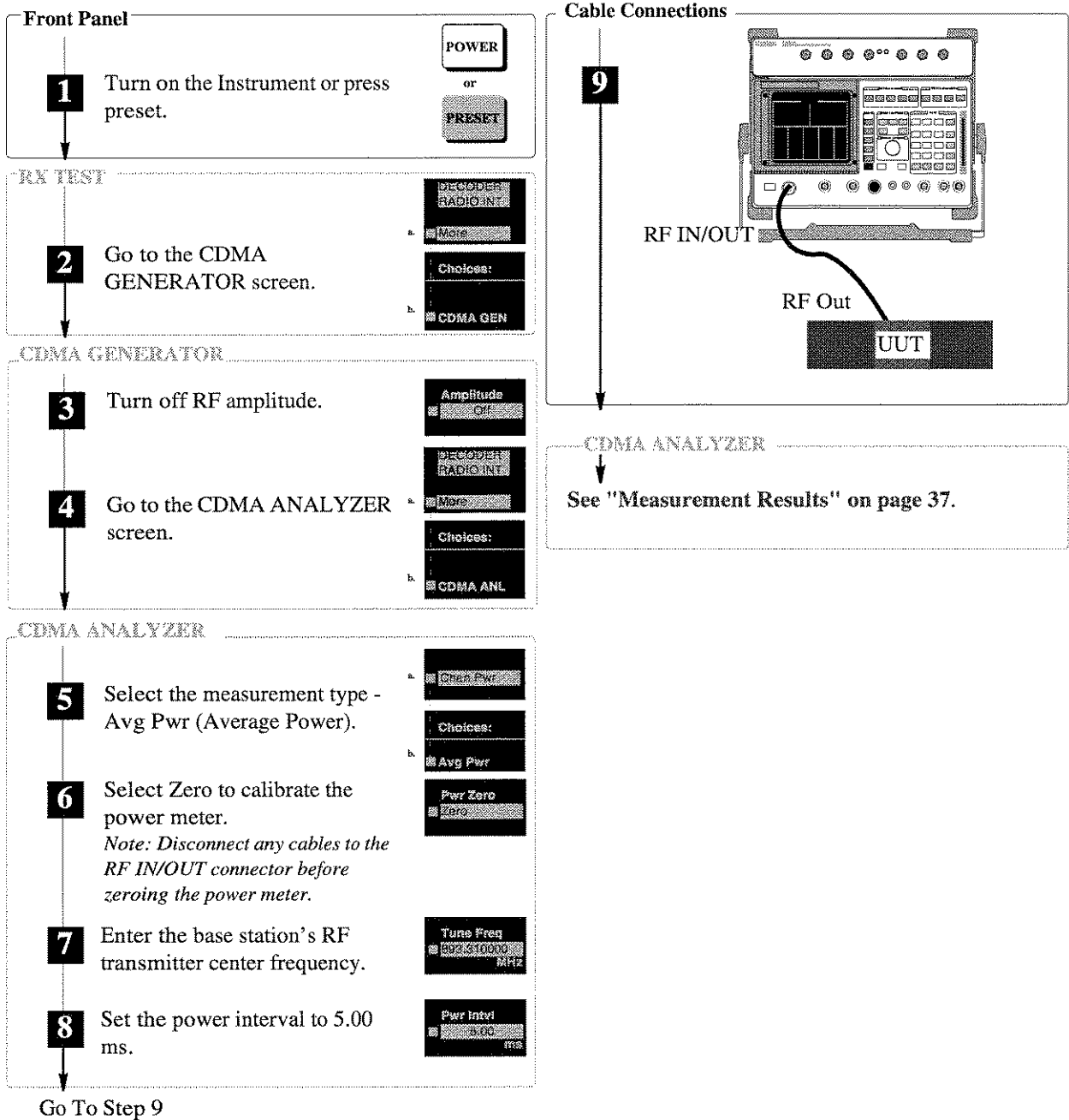
Figure 1 Average Power Measurement Procedure
