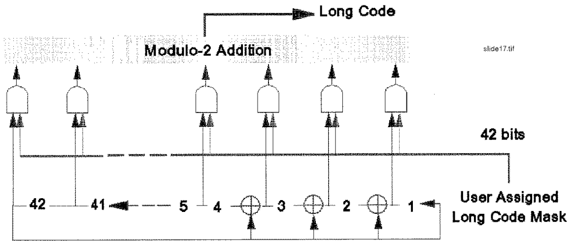
Figure 22 Long Code Generation
